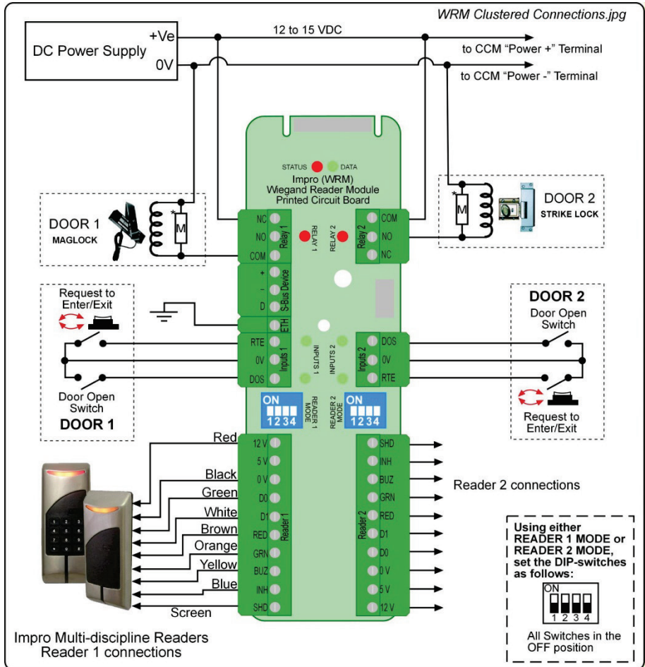
Figure 4: Typical Clustered Impro WRM Electrical Connections
